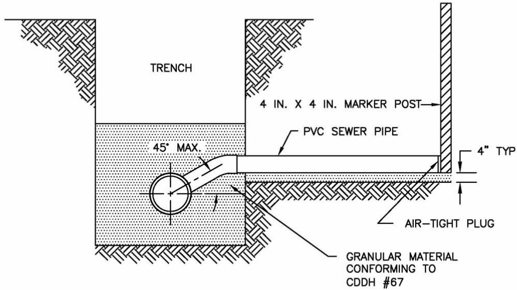
CROSS SECTION
